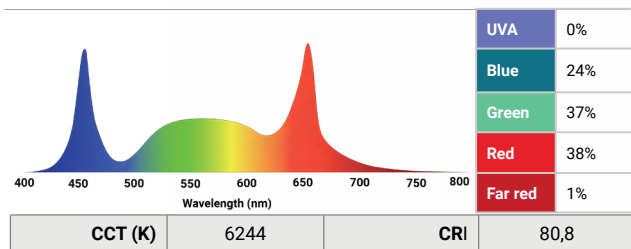
helioSPEC R60
