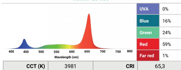
helioSPEC R80
